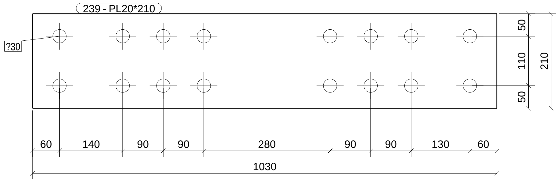
FRONT VIEW
